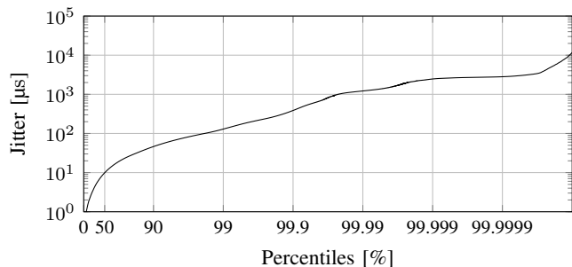
Fig. 8: HDR-histogram over all jitter values of all 100 topologies
